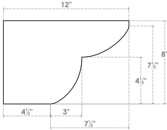
SIDE PROFILE
